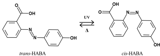
Fig. 2 Trans-cis isomerization of push-pull azo dye HABA.
