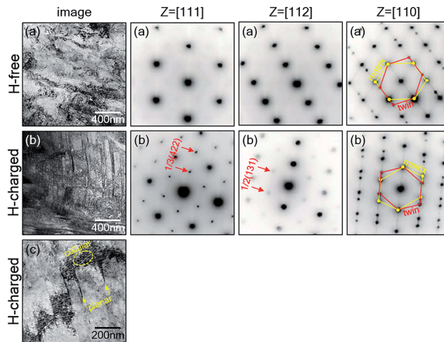
Fig. 8 Bright-field TEM images and selected area electron diffraction (SAED) patterns of 316L SS after RT tensile tests at a strain rate of 2 \times 10^{-6} s^{-1} . (a) H-Free, (b) H-charged, (c) H-charged and 10% tensile deformed.
