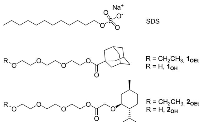
Fig. 1 A typical sulfonate surfactant and the new “reverse” surfactants 1_{\text{OEt}} , 2_{\text{OEt}} and 1_{\text{OH}} , 2_{\text{OH}} .
