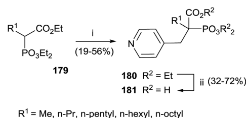
Fig. 5 Phophonocarboxylates.
