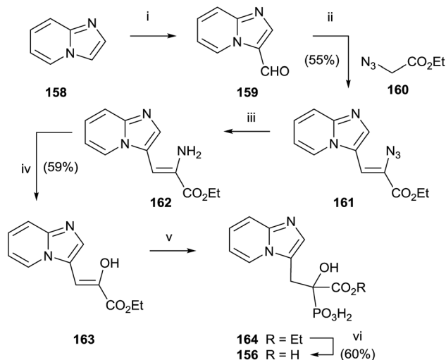
Fig. 5 Phophonocarboxylates.
