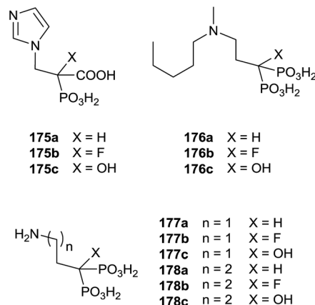
Fig. 5 Phophonocarboxylates.
