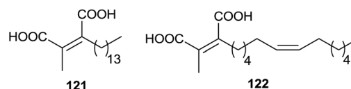
Fig. 3 Chaetomelic acids.
