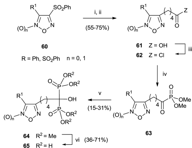
Scheme 15 Reagents and conditions: (i) 1,5-pentanediol, NaOH 50% w/w, THF. (ii) Jones reagent, acetone, 0 °C to rt. (iii) SOCl 2 . (iv) P(OMe) 3 , dry THF, 0 °C to rt. (v) HPO(OMe) 2 , Et 3 NH, dry THF, 0 °C to rt; (vi) TMSBr, CH 2 Cl 2 ; then MeOH, 0 °C to rt.
