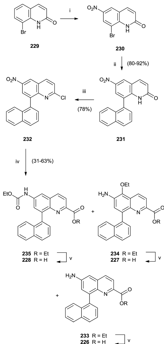
Scheme 39 Reagents and conditions: (i) fuming HNO 3 , TFA, from 0 °C to rt. (ii) K 2 CO 3 , boronic acid, [(C 6 H 5 ) 3 P] 2 PdCl 2 , DMF/H 2 O, 80–92 °C. (iii) POCl 3 , Et 4 NCl, N,N -dimethylaniline, CH 3 CN. (iv) CO, [(C 6 H 5 ) 3 P] 2 PdCl 2 , Et 3 N, EtOH, 110 °C. (v) LiOH, H 2 O/dioxane.
