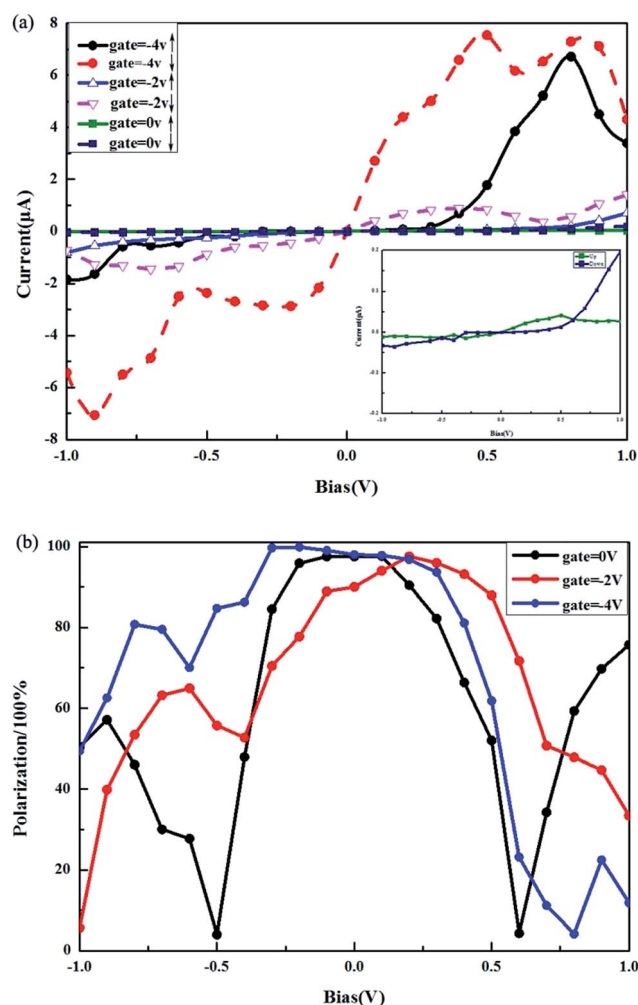
Fig. 4 (a) shows the calculated spin-dependent current-voltage characteristics for the (ZBNNR) 5 -(ZGNR) 3 -B v device under different V_g s ( V_g = -4 V, -2 V, 0 V), respectively. Inset: the amplified I - V curve of (ZBNNR) 5 -(ZGNR) 3 -B v device under V_g = 0 V. (b) shows the spin-filter efficiency (SFE) as a function of the electric field intensity and bias for (ZBNNR) 5 -(ZGNR) 3 -B v device, V_g = -4 V, -2 V, 0 V, respectively.
