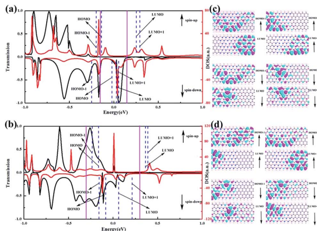
Fig. 5 (a)–(b) shows the spin-dependent transmission spectra and the electronic density of states of (ZBNNR) 5 –(ZGNR) 3 –B v device at V_g = -4 V with V_b = -0.3 V, 0.6 V, respectively. The vertical solid purple lines stand for bias window, and the dashed blue lines represent the spin-polarized Frontier molecular orbitals. (c)–(d) shows the MPSH of the corresponding spin-dependent HOMO–1, HOMO, LUMO and LUMO+1 under bias of -0.3 V and 0.6 V, respectively.
