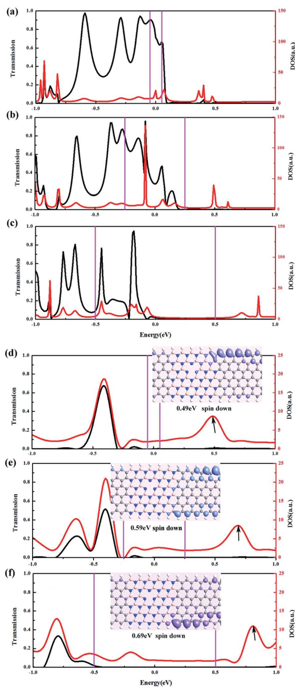
Fig. 6 Transmission spectra and electronic density of states of (ZBNNR) 5 –(ZGNR) 3 –B v device for spin down channel. (a)–(c) represents V_b = 0.1 V, 0.5 V and 1.0 V at V_g = -4 V, respectively. (d)–(f) represents V_b = 0.1 V, 0.5 V and 1.0 V at V_g = 0.0 V, respectively. Their LDOS are shown in the corresponding insets with an isovalue of 0.03. The region between the vertical purple lines is the bias window.
