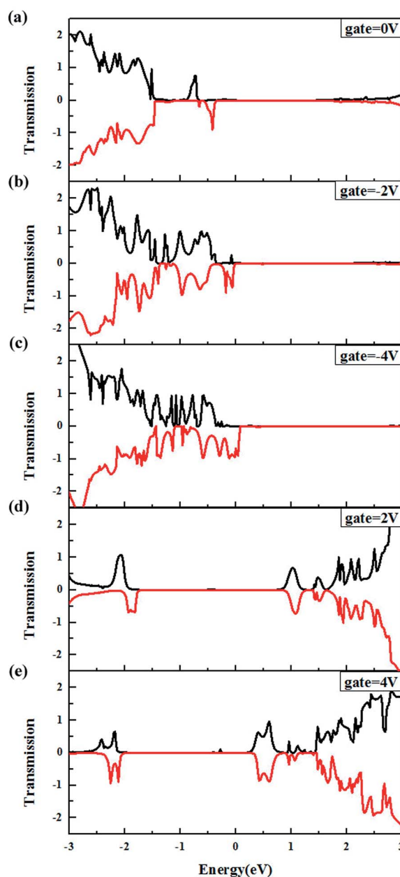
Fig. 2 (a)–(e) shows the spin-dependent transmission spectra of (\text{ZBNNR})_5\text{--}(\text{ZGNR})_3\text{--B}_v FET device at V_g = 0 V, -2 V, -4 V, 2 V, 4 V with V_b = 0 V, respectively.
