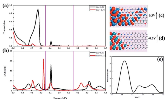
Fig. 7 (a) Transmission spectrum, (b) projected density of states (black line for 0.3 V, red line for -0.3 V) of (\text{ZBNNR})_5-(\text{ZGNR})_3-B_V devices for spin up channel under the applied gate V_g = -4 V. (c) and (d) represents the corresponding transmission eigenstates at the Fermi level. (e) RR for the spin up channel, and the solid purple lines indicate the bias window.
