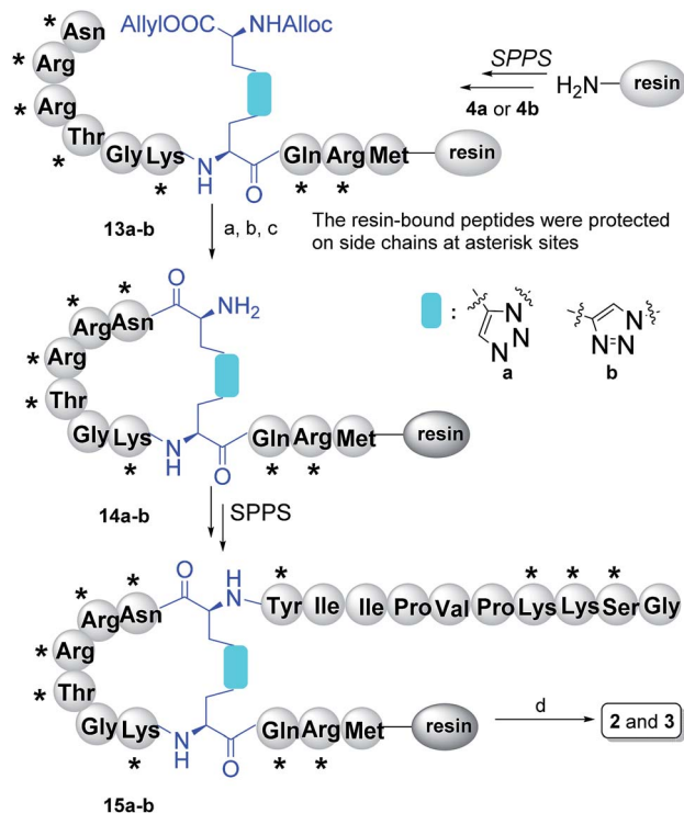
Scheme 3 Reagents and conditions: (a) \text{Pd}(\text{PPh}_3)_4 , \text{PhSiH}_3 ; (b) 20% piperidine/DMF; (c) PyAOP, HOAt, NMM, NMP; (d) TFA/TIPS/ \text{H}_2\text{O} (95 : 2.5 : 2.5, v/v/v), 29.7% for 2 and 34.5% for 3. The following protecting groups for amino acid side chains were used: tert -butyl (tBu; for Thr, Tyr and Ser), 2,2,4,6,7-pentamethyldihydrobenzo-furane-5-sulfonyl (pbfi; for Arg), tert -butoxycarbonyl (Boc; for Lys) and trityl (Trt; for Gln, Asn).
