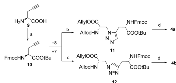
Scheme 2 Reagents and conditions: (a) (i) Fmoc-OSU, Na 2 CO 3 , H 2 O/1,4-dioxane; (ii) t BuOH, DCC, DMAP, DCM, 70.0% in 2 steps; (b) (i) 8 , [Cp*RuCl(COD)], DMF, 40 °C; (ii) H 2 , 10% Pd/C, MeOH; (iii) Alloc-Cl, Na 2 CO 3 , H 2 O/CH 3 CN; (iv) allyl bromide, NaHCO 3 , DMF, 54.7% in 4 steps; (c) 7 , CuI, DIPEA, DMF, 84.1%; (d) TFA/DCM, 95.0% for 4a and 96.3% for 4b .
