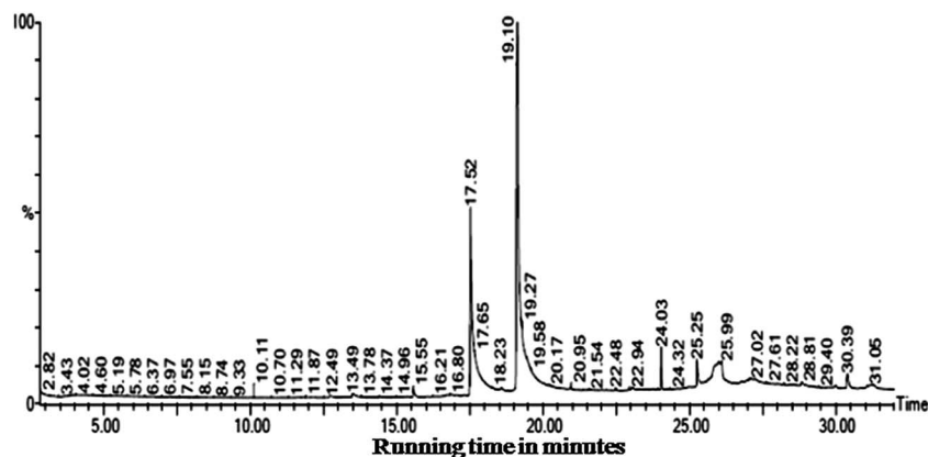
Fig. 3 The insecticidal compounds identified in the ethyl acetate mycelium extracts obtained from B. bassiana .
