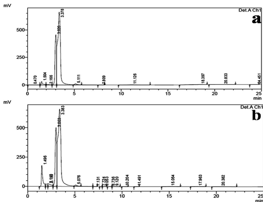
Fig. 4 (a) The HPLC chromatogram of the n -hexadecanoic acid standard and (b) the HPLC chromatogram of the ethyl acetate mycelium extract obtained from B. bassiana .
