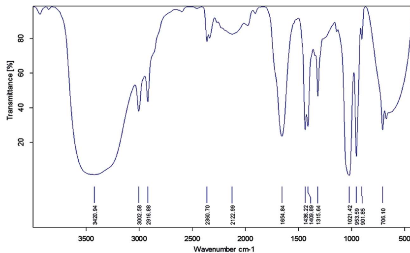
Fig. 2 FTIR analysis of the ethyl acetate mycelia extract obtained from B. bassiana .
