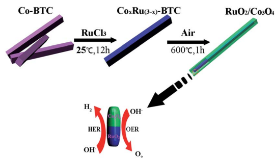
Scheme 1 Synthetic route for RuO 2 /Co 3 O 4 .
