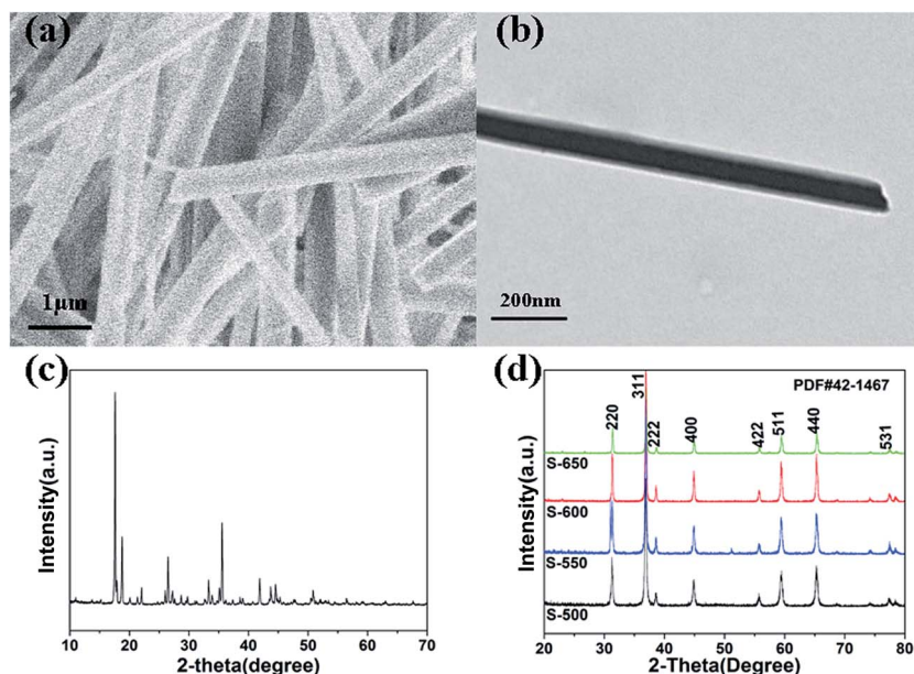
Fig. 1 (a) SEM image of Co-BTC. (b) TEM image of Co-BTC. (c) XRD patterns of Co-BTC. (d) XRD patterns of the Co 3 O 4 samples (S-650, S-600, S-550, S-500).
