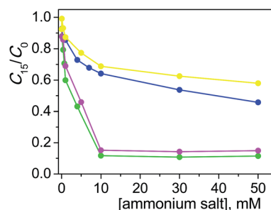
Fig. 4 Photodegradation of ARS (0.20 mM) with \text{TiO}_2 ( 0.4 \text{ g l}^{-1} ) at pH 12 after 15 min of irradiation as a function of TPABr (●), BPyBr (●), ASBr (●), BQBr (●) concentration.
