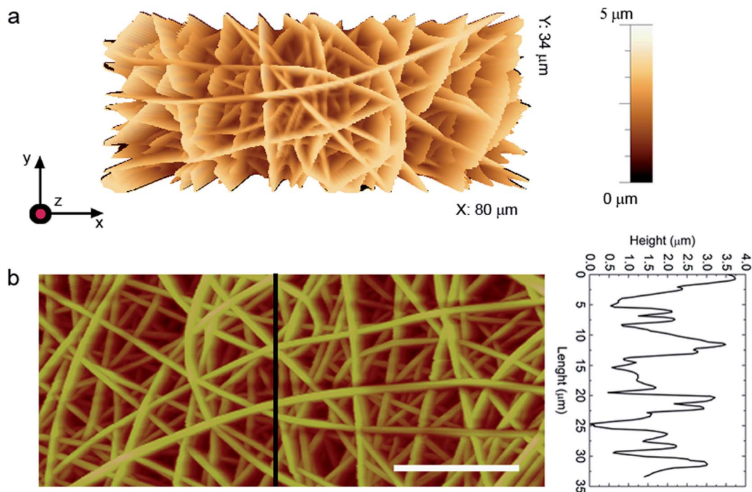
Fig. 3 AFM topographic micrograph of a fiber mat (2-R g ). (a) 3D view. (b) 2D view. Scale bar: 20 \mu\text{m} . Vertical scale: 5 \mu\text{m} . The height profile is taken along the line highlighted in the planar view.
