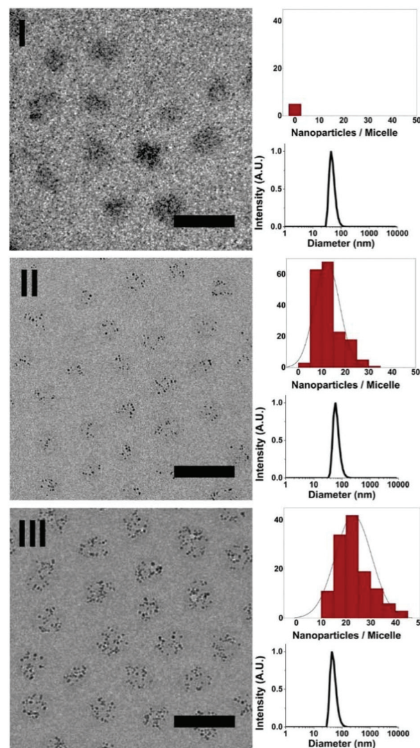
Fig. 1 Dendrimicelle characterization. In each panel, the figure on the left shows a cryoTEM image, and the figures on the right show the counted nanoparticles per micelle (upper), and number-averaged DLS size plot (lower). Dendrimicelles made from: top (I) empty dendrimers. The contrast observed originates from the dense dendrimicelle cores. Middle (II), from 50% Au 256 -filled and 50% empty dendrimers; they contain 12 \pm 5 AuNPs per micelle, and an equal amount of empty dendrimers which are not individually observable. Bottom (III), from Au 256 -filled dendrimers. The dendrimicelles contain 23 \pm 7 AuNPs per micelle. The AuNPs encapsulated inside the dendrimers greatly improve the contrast of the TEM images (of II and III) and allow for determining aggregation numbers. Scale bars are 50 nm.
