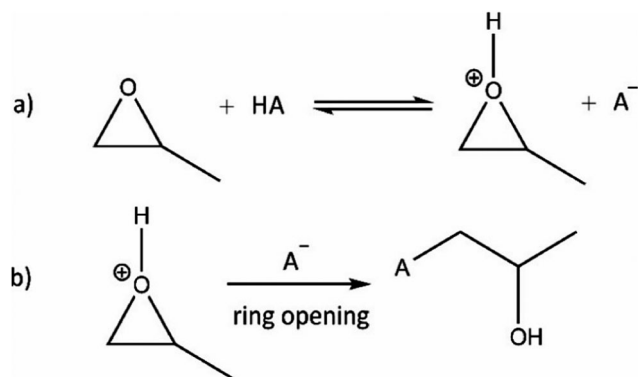
Fig. 5 Reaction schematics for propylene oxide as proton scavenger. In a first step, (a) propylene oxide gets protonated by the acid HA and (b) in a second step the acid anion induces a ring opening reaction through a nucleophilic attack.
