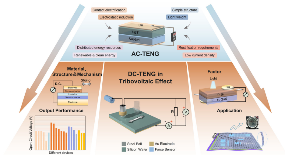
Fig. 1 Schematic illustration of the AC-TENG and DC-TENG based on the tribovoltaic effect.
