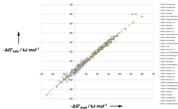
Fig. 14 Comparison of free energies calculated using the SSIP model developed here ( -\Delta G_{\text{calc}}^\circ ) with experimental values ( -\Delta G_{\text{expt}}^\circ ) for transfer of 219 different solutes from water to 35 solvents (overall rmsd is 1.4 kJ mol -1 for 1713 data points). The red line is y = x .
