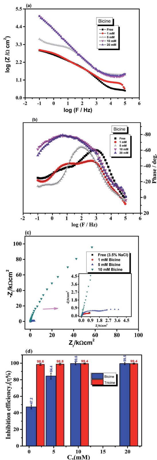
Fig. 6 (a–c) Bode and Nyquist diagrams for copper in 3.5% NaCl solutions with different concentrations of bicine at 25 °C. (d) Variation of the corrosion inhibition efficiency of Cu corrosion in stagnant naturally aerated neutral 3.5% NaCl solutions with the bicine and tricine concentration at 25 °C obtained from the EIS measurements.
