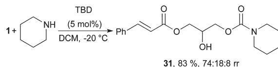
Scheme 4 Organocatalytic ring opening of 1 to form acyclic carbamate 31 . 1 (0.2 mmol), piperidine (1.2 eq.), isolated yield, regioisomeric ratio determined by ^1\text{H} NMR of crude material, major isomer separable by flash chromatography.
