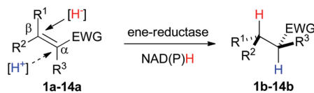
Scheme 2 Bioreduction of activated alkenes 1–14a by ene-reductases at the expense of nicotinamide cofactor.
