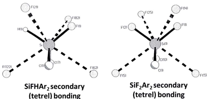
Fig. 11 Crystal structure of \text{SiFHA}_2 , \text{Ar} = \text{C}_6\text{H}_2(\text{CF}_3)_3 (top), with secondary (tetrel) bonding shown as dashed bonds and primary bonding (solid lines) and secondary bonding (dashed lines) at Si in \text{SiFHA}_2 and \text{SiF}_2\text{Ar}_2 (bottom). Secondary (tetrel) \text{Si}\cdots\text{F} bonds are longer than primary (covalent) \text{Si}\text{--}\text{F} bonds. Secondary bonds trans to F are shorter than those trans to C. Adapted from ref. 57 with permission from Elsevier.
