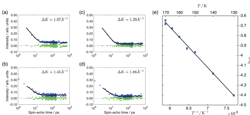
Fig. 2 Polarisation measurements as a function of the spin-echo time, t , for 0.03 ML (panels a, c) and 0.1 ML (panels b, d) of benzene/Cu(111). The different panels show the measurements at the indicated momentum transfers and a temperature of 170 K. The experimental data are plotted as blue points, a single exponential of the form f(t) = a \exp(-\alpha t) + c from 3 ps is shown as a black line and the residual after subtracting the exponential from the data as green points. The data at times smaller than 3 ps is excluded as it is influenced by the initial fast decay described in the text. Panel (e) shows the temperature dependence of the dephasing rate for a coverage of 0.03 ML at \Delta K = 0.3 \text{ \AA}^{-1} as an Arrhenius plot. The solid line illustrates the fit to an Arrhenius form, resulting in an effective activation energy of 35 \pm 1 \text{ meV} . All the data were measured along the [11\bar{2}] direction.
