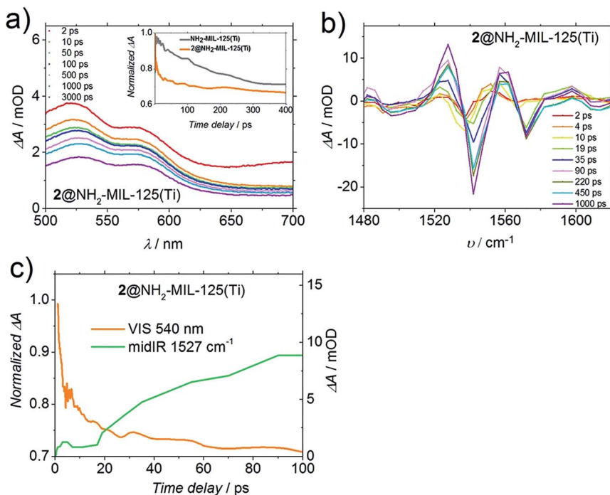
Fig. 6 (a) Differential transient spectra of 2@ \text{NH}_2 -MIL-125(Ti) in DMF upon excitation at 400 nm, inset: comparison of the time traces of \text{NH}_2 -MIL-125(Ti) and 2 occluded in \text{NH}_2 -MIL-125(Ti) at 540 nm in DMF, (b) differential transient absorption mid-IR spectra for 2@ \text{NH}_2 -MIL-125(Ti) in DMF upon excitation at 400 nm, and (c) representative time traces of 2@ \text{NH}_2 -MIL-125(Ti) upon excitation at 400 nm in DMF recorded at 1527 \text{cm}^{-1} (green). The orange line (corresponding to the left axis) represents the time traces at 540 nm in DMF (same as in (a), inset orange line).
