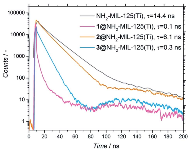
Fig. 5 Time resolved fluorescence of \text{NH}_2 -MIL-125(Ti) in water (grey), 1@ \text{NH}_2 -MIL-125(Ti) in acetonitrile (pink), 2@ \text{NH}_2 -MIL-125(Ti) in DMF (orange) and 3@ \text{NH}_2 -MIL-125(Ti) in water (blue). The suspensions were excited by a 404 nm laser. The decrease in fluorescence over time was measured at a wavelength of 430 nm and fitted by a sum of exponential decays (only the fastest \tau component, which is the biggest contribution, is shown for clarity).
