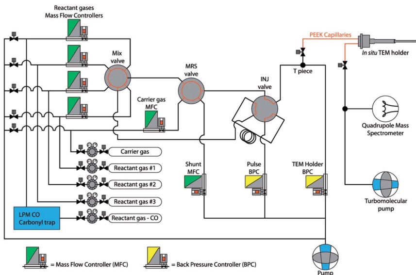
Fig. 2 Schematic overview of the gas supply system, showing the computer operated Mass Flow Controllers (MFCs), Back Pressure Controllers (BPCs), and rotating mixing valves.
