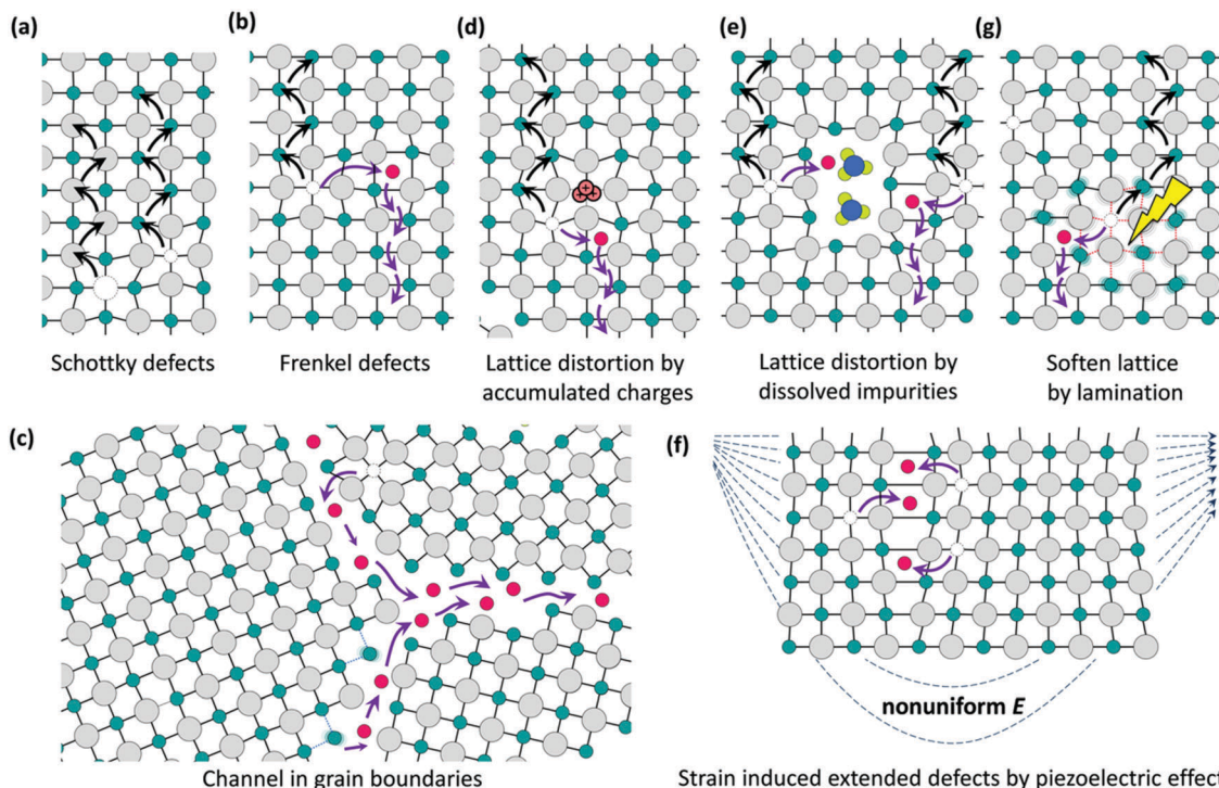
Fig. 16 Schematic diagrams illustrating the ionic migration channels. (a) Schottky defects, or vacancies; (b) Frenkel defects, or interstitials. (c) Ion migration at the grain boundaries. Distortion of the lattice due to (d) accumulation of charges, (e) impurities, (g) light-illumination-induced lattice softening, and (f) piezoelectric effects. Reproduced from ref. 153. Copyright ©2016 American Chemical Society.
