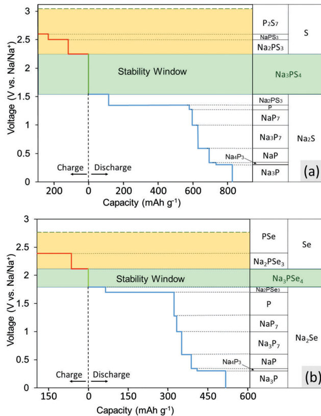
Fig. 2 Calculated stability window and decomposition products for (a) Na 3 PS 4 and (b) Na 3 PSe 4 . The green shaded region is the thermodynamically stable voltage window, and the yellow shaded region is the additional voltage range that could be kinetically stabilized.
