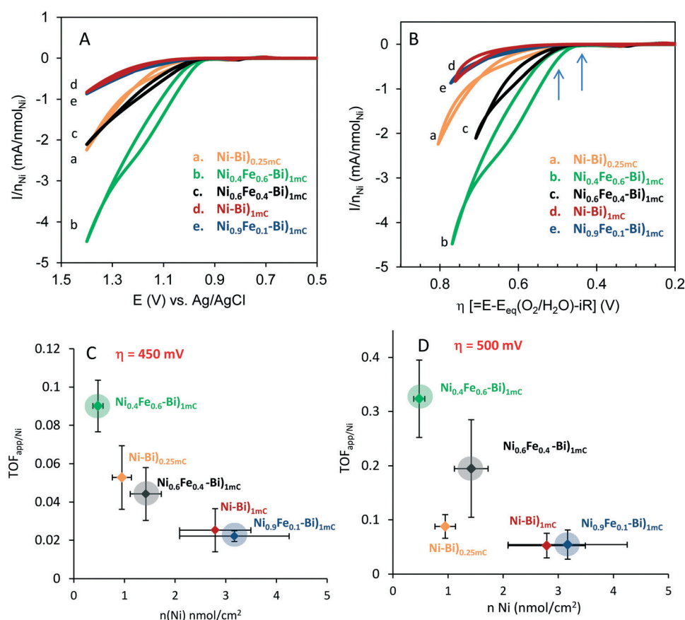
Fig. 2 Current divided per n_{\text{Ni}} versus potential (CVs in Fig. 1) (A) and versus overpotential \eta (B) for as-deposited \text{Ni-Bi}_{0.25\text{mC}} (a), \text{Ni}_{0.4}\text{Fe}_{0.6}\text{-Bi}_{1\text{mC}} (b), \text{Ni}_{0.6}\text{Fe}_{0.4}\text{-Bi}_{1\text{mC}} (c), \text{Ni-Bi}_{1\text{mC}} (d) and \text{Ni}_{0.9}\text{Fe}_{0.1}\text{-Bi}_{1\text{mC}} (e). Apparent turnover frequency per Ni center ( \text{TOF}_{\text{app}}/\text{Ni} ) versus nmol \text{cm}^{-2} of Ni measured at 3 films each of \text{Ni-Bi}_{0.25\text{mC}} , \text{Ni}_{0.4}\text{Fe}_{0.6}\text{-Bi}_{1\text{mC}} , \text{Ni}_{0.6}\text{Fe}_{0.4}\text{-Bi}_{1\text{mC}} , \text{Ni}_{0.9}\text{Fe}_{0.1}\text{-Bi}_{1\text{mC}} , and \text{Ni-Bi}_{1\text{mC}} at \eta = 450\text{ mV} (C) and \eta = 500\text{ mV} (D); the points for films with co-deposited Fe have shaded circles for emphasis. The arrows in panel B refer to the overpotentials for the TOF in (C) and (D).
