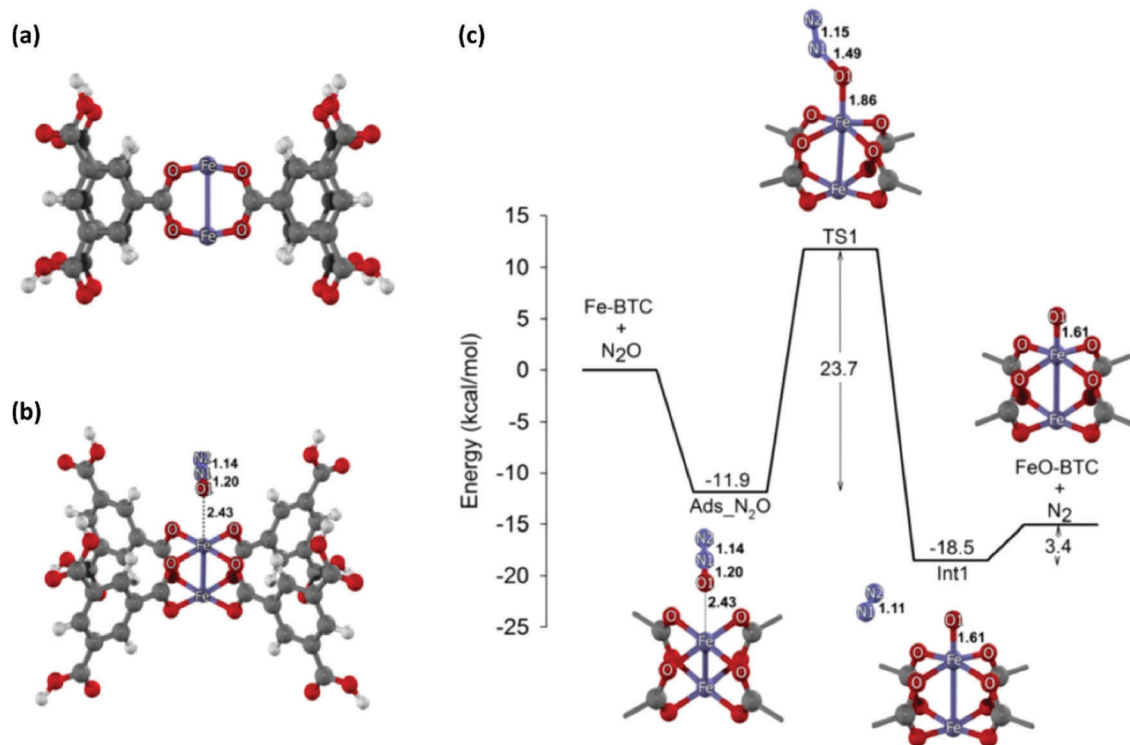
Fig. 19 (a) and (b) Optimised structures of the (a) FeBTC model and (b) its interaction with nitrous oxide; (c) energy profile and some geometric parameters of reactants, intermediate, and transition state involved in the decomposition of N 2 O over FeBTC (distances in Å). Figure adapted from ref. 289 with permission of Wiley, copyright 2016.
