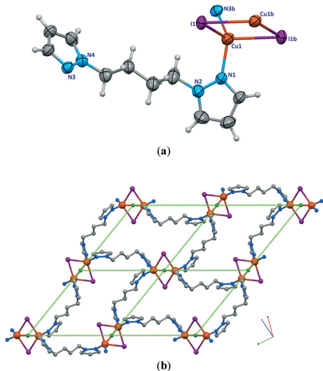
Fig. 2 The structure of [\text{Cu}(\mu_2\text{-I})(\mu\text{-bpmb})]_n (1b). (a) Asymmetric unit of 1b with additional atoms to complete the coordination of Cu. (b) Part of the two-dimensional 4^4\text{-sql} net structure with four equal parallelograms.
