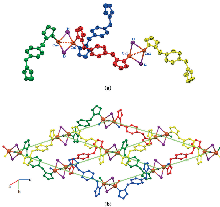
Fig. 3 The structure of [\text{Cu}(\mu_2\text{-I})(\mu\text{-bpmb})]_n (2). (a) Asymmetric unit of 2 with labeling scheme for Cu and I. (b) Part of the two-dimensional structure with four crystallographically independent \mu\text{-bpmb} linkers shown in different colors.
