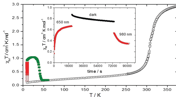
Fig. 4 Thermal behaviour of the \chi_{\text{M}}T values for 1 in the dark ( \circ ), under a 650 nm irradiation ( \Delta ) and after this irradiation in the dark at 0.4 \text{ K min}^{-1} ( \blacksquare ). The inset reports the time dependence of the \chi_{\text{M}}T values in 1 following irradiation at 650 nm ( \blacktriangle ) and 980 nm ( \blacktriangledown ) compared to the relaxation in the dark at 10 K ( \blacksquare ).
