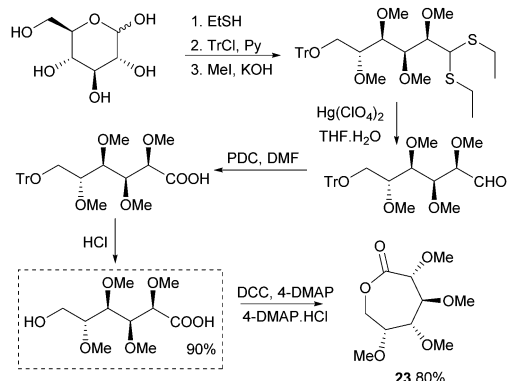
Fig. 14 Synthesis of \omega -hydroxyacid precursor and lactone 23 via D-glucose diethylmercaptapyl intermediate.
