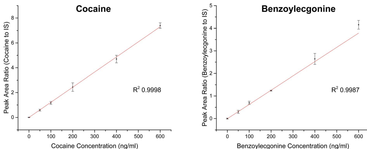
Fig. 3 Calibration curve for cocaine ( m/z 182 ) and benzoylecgonine ( m/z 168 ) in pooled urine analysed using Plate Express™ coupled with an expression compact mass spectrometer (CMS) with cocaine- d_3 ( m/z 185 ) internal standard.
