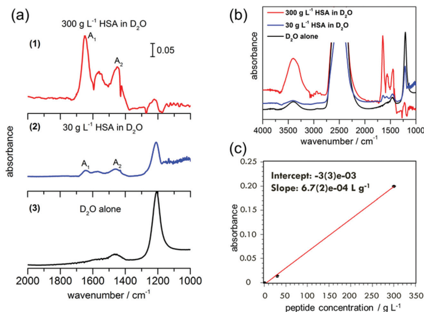
Fig. 4 (a) ATR-IR spectra of (1) HSA in D 2 O (300 g L -1 ), (2) HSA in D 2 O (30 g L -1 ) in 10 nm deep Ge ATR-IR nanochannel devices and (3) bulk D 2 O alone obtained on the Ge ATR-IR crystal. A 1 (1649 cm -1 ) and A 2 (1450 cm -1 ) indicate the amide I and amide II peaks, respectively. (b) The extended spectra of the same, from 4000 to 1000 cm -1 . (c) Peak absorbance of amide I mode versus concentration.
