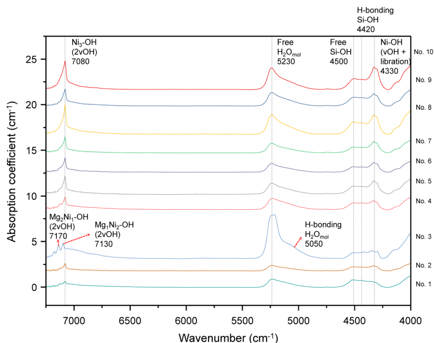
Fig. 4 Near-infrared (NIR) absorption spectra (absorption coefficient, cm −1 ) of the ten chrysoprase samples. Key bands are labelled and assigned as follows: \sim 7080 cm −1 (first overtone of Ni–OH stretching, with minor overlap from Si–OH and H 2 O overtones), \sim 5230 cm −1 (combination band of non-hydrogen-bonded molecular water), \sim 4500 cm −1 (isolated Si–OH + siloxane framework vibrations), \sim 4420 cm −1 (siloxane framework bending + strongly H-bonded germinal silanol), and \sim 4330 cm −1 (Ni–OH combination band showing partial splitting).
