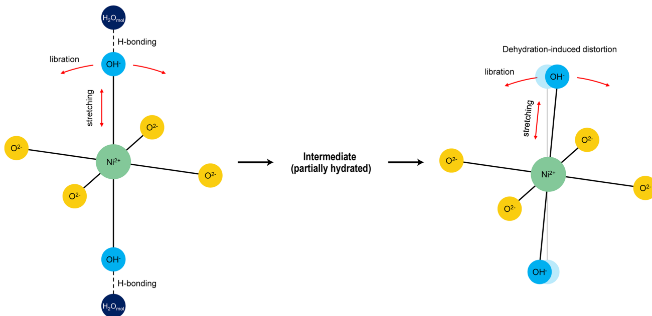
Fig. 9 Schematic illustration of the \text{Ni}^{2+} coordination environment before (left), during (center), and after (right) dehydration. In the hydrated state (pimelite-like), interlayer water molecules form hydrogen bonds with \text{OH}^- groups, stabilising the \text{Ni-OH} octahedra and maintaining a relatively symmetric crystal field. The intermediate state represents a partially dehydrated condition, in which most \text{Ni-OH} groups remain hydrogen-bonded while a fraction lose hydrogen bonding, leading to incipient distortions. In the anhydrous state (willemseite-like), the complete loss of hydrogen bonding induces significant structural distortions, resulting in multiple non-equivalent \text{Ni-OH} environments. These variations lead to slightly different vibrational frequencies of the \text{Ni-OH} stretching and libration modes, which together contribute to the observed splitting of the \sim 4330\text{ cm}^{-1} combination band in the near-infrared absorption spectra.
