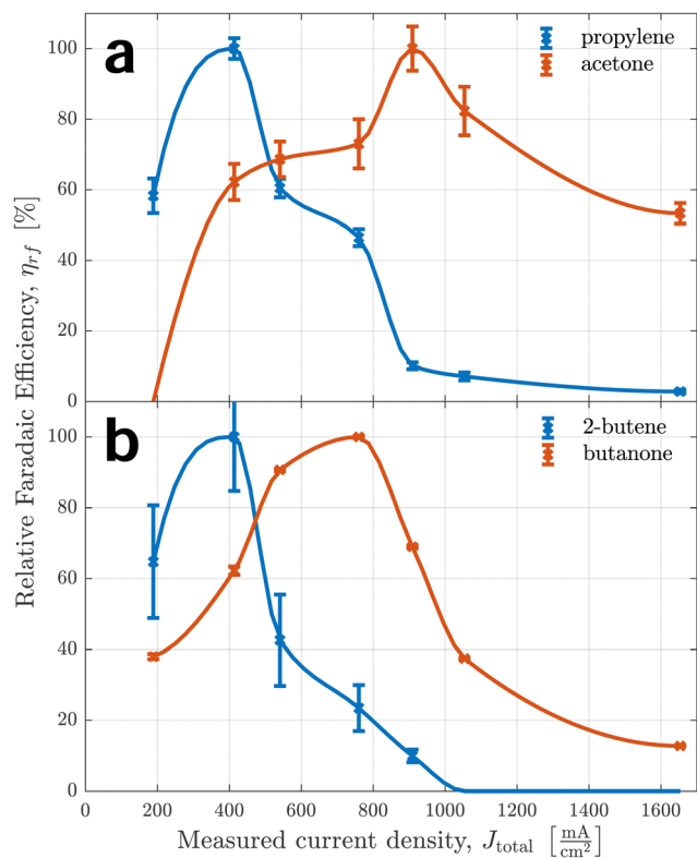
Fig. 6 Relative faradaic efficiencies of alk-2-enes and ketones in comparison. The top graph (a) shows selectivity trends of corresponding \text{C}_3 products and the bottom graph (b) of \text{C}_4 products.
