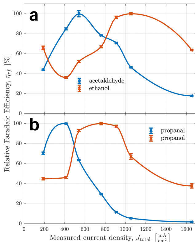
Fig. 7 Relative faradaic efficiencies of aldehydes and primary alcohols in comparison. The top graph (a) shows selectivity trends of corresponding \text{C}_2 products and the bottom graph (b) of \text{C}_3 products.
