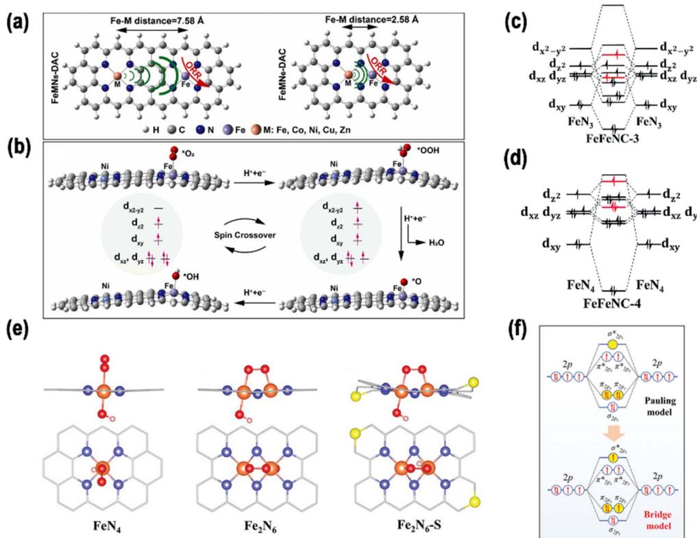
Fig. 6 (a) Structures of FeMN 6 -DAC and FeMN 8 -DAC. (b) Side perspective of reaction intermediates of FeNiN 8 -DAC in the ORR. Reproduced with permission. 60 Copyright 2023, Elsevier. Orbital interactions between Fe atoms in (c) FeFeNC-3 and (d) FeFeNC-4. Reproduced with permission. 84 Copyright 2022, the Royal Society of Chemistry (e) geometric models of FeN 4 , Fe 2 N 6 , and Fe 2 N 6 -S with absorbed O 2 . (f) Schematic representation of the potential electron orbital configurations of O 2p orbitals in various oxygen-adsorption arrangements. Reproduced with permission. 85 Copyright 2023, Wiley-VCH.
