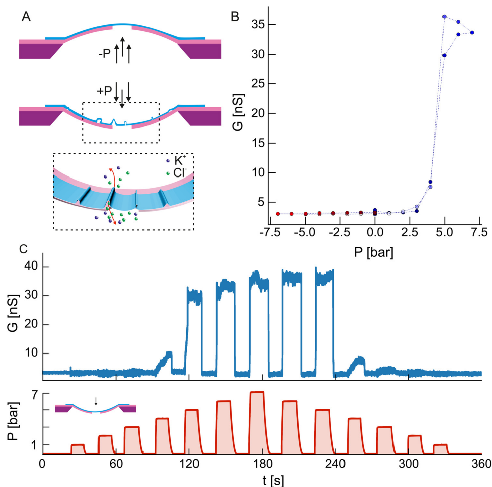
Fig. 2 Delamination of suspended \text{MoS}_2 due to pressure induced surface indentation. (A) Toy model demonstrating bulging (top) and indentation (bottom) of the membrane under positive and negative hydraulic pressure gradients. The bottom inset shows the proposed mechanism for the formation of conductive channels between two sides of the membrane due to local wrinkling and detachment of the \text{MoS}_2 . (B) Conductance G of the sample was obtained through ionic current measurements at 100 mV at different values of the pressure gradient P applied to the membrane. The measurement protocol involved subsequent measurements at different pressure values followed by a measurement at P = 0 bar to confirm that the baseline value has not changed. Panel (C) shows the time traces of the pressure P and conductance G as shown in panel b. Note that only positive pressure gradient values are shown to emphasize the abrupt increase in conductance seen in panel b.
