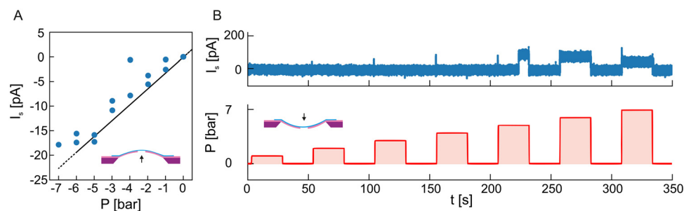
Fig. 3 Streaming measurements on suspended \text{MoS}_2 during delamination. (A) Streaming current I_s as measured on the sample shown in Fig. 2b and c during the membrane bulging state. No external potential was applied to the sample (closed circuit measurement). (B) Anomalous increase of streaming current I_s for positive pressures matching the delaminating state in Fig. 2b and c. The top panel shows the time trace of the measured streaming current I_s , while the bottom panel shows the applied pressure gradient P .
