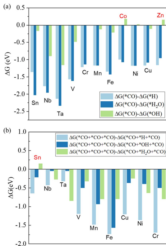
Fig. 3 Adsorption energy differences between CO and: (a) hydrogen, hydroxide ions, and H 2 O at Mo sites; (b) hydrogen, hydroxide ions, and H 2 O at dopant sites.
