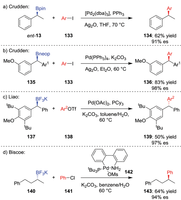
Scheme 19 Enantiospecific transition-metal-mediated sp^2 – sp^3 cross-coupling of unactivated secondary boronic esters and trifluoroborate salts. Ar = p - \text{ClC}_6\text{H}_4 , Ar 1 = p - \text{CH}_3\text{CH}_2\text{C}_6\text{H}_4 , Ar 2 = p - \text{CH}_3\text{C}_6\text{H}_4 , Ms = \text{CH}_3\text{SO}_2 , neop = neopentyl glycol.
