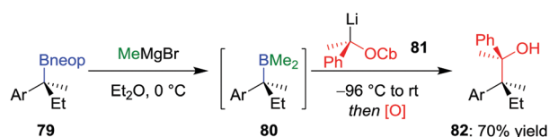
Scheme 12 Lithiation–borylation reactions of enantioenriched boronic esters to form quaternary–quaternary contiguous stereogenic centres. OCb = N,N -diisopropylcarbamate, Ar = p -OMeC 6 H 4 , neop = neopentyl glycol.
