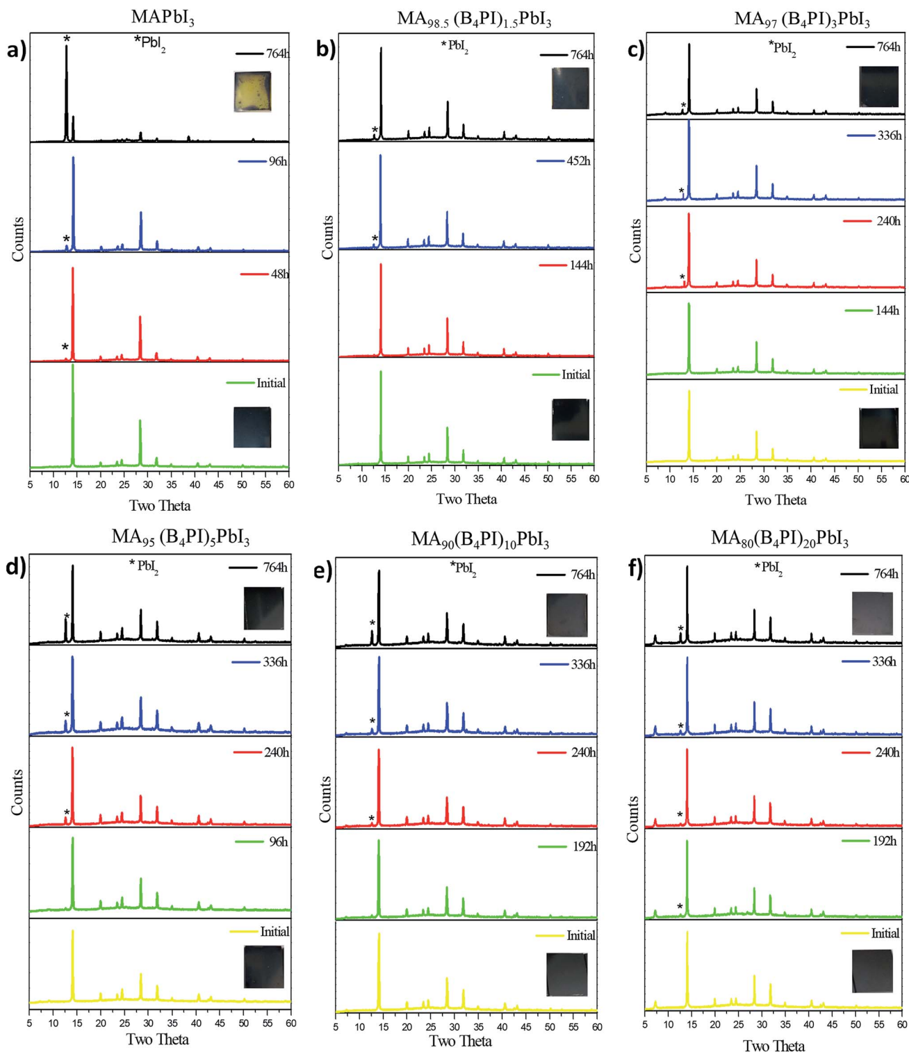
Fig. 7 XRD of film degradation: (a) pristine \text{MAPbI}_3 ; (b–f) \text{MA}_{1-x}(\text{B}_4\text{PI})_x\text{PbI}_3 .
