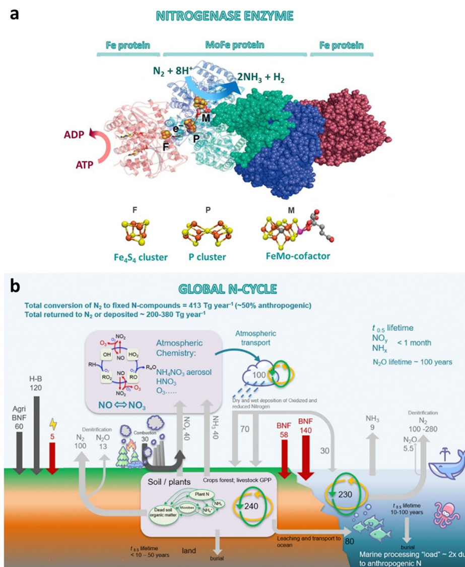
Fig. 4 (a) Structure of the nitrogenase enzyme complex, including the MoFe and Fe protein components with the three metaloclusters ( Fe_4S_4 cluster, P cluster and FeMo-cofactor). The Figure also shows the ATP hydrolysis by the Fe protein, the electron transfer to the catalytic site, and the biological nitrogen fixation to ammonia (adapted from ref. 48). (b) Global nitrogen cycle and fluxes in Tg per year (BNF, biological nitrogen fixation; H-B, Haber-Bosch nitrogen fixation; GPP, gross primary productivity). Reproduced with permission from MacFarlane et al. 49 Copyright 2020 Elsevier Inc.
