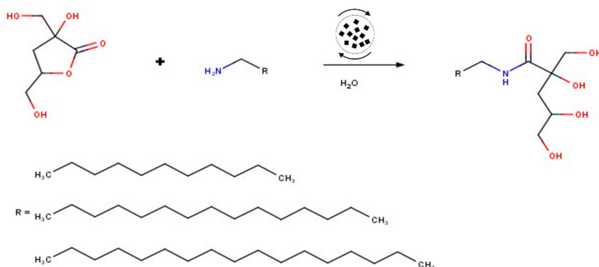
Fig. 1 Reaction scheme between GISA L and amides of different chain lengths.
