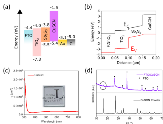
Fig. 1 (a) The energy level diagram of each layer in the FTO/ \text{TiO}_2 / \text{Sb}_2\text{S}_3 /CuSCN/Au (or carbon) solar cells. (b) SCAPS-1D modeling determined energy band diagram of the solar cells at short circuit. (c) The absorption coefficient of a CuSCN thin film on a glass substrate. (d) X-Ray diffraction pattern of commercial CuSCN powder and the prepared CuSCN film on the FTO substrate.
