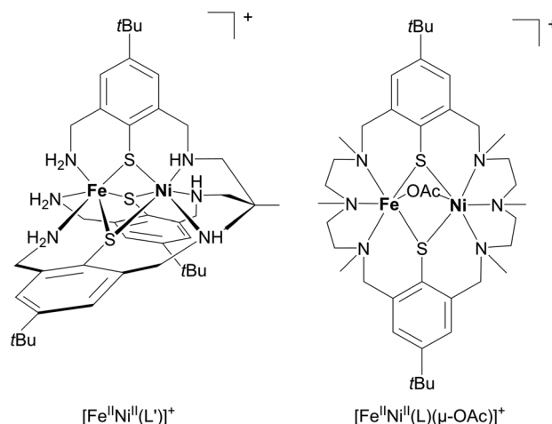
Fig. 1 Heterobinuclear \text{Fe}^{\text{II}}\text{Ni}^{\text{II}} complexes supported by compartmental amino-thiophenolato ligands. The [\text{Fe}^{\text{II}}\text{Ni}^{\text{II}}\text{L}]^+ complex has been reported previously. 49
