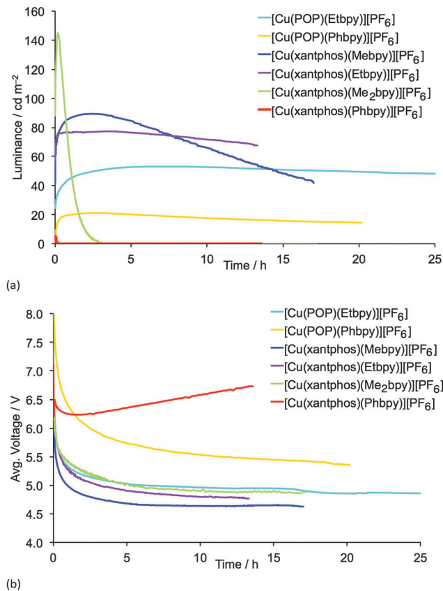
Fig. 10 Luminance (a) and average voltage (b) for ITO/PEDOT:PSS/[Cu(P A P)(N A N)][PF 6 ]:[Emim][PF 6 ] 4:1 molar ratio/Al LECs measured using a pulsed current driving (average current density 50 A m -2 , 1 kHz, 50% duty cycle, block wave). [Emim][PF 6 ] = 1-ethyl-3-methylimidazolium hexafluoridophosphate.
