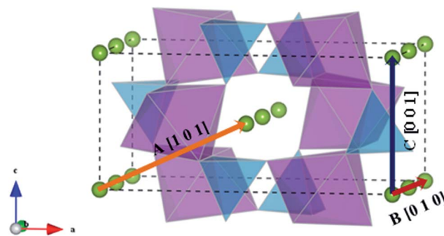
Fig. 3 Schematic representation of the possible migration paths in olivine-type \text{AFEPo}_4 ( A = \text{Li}^+ or \text{Na}^+ ). Blue: \text{PO}_4 tetrahedra; purple: \text{FeO}_6 octahedra; green: Li/Na.
