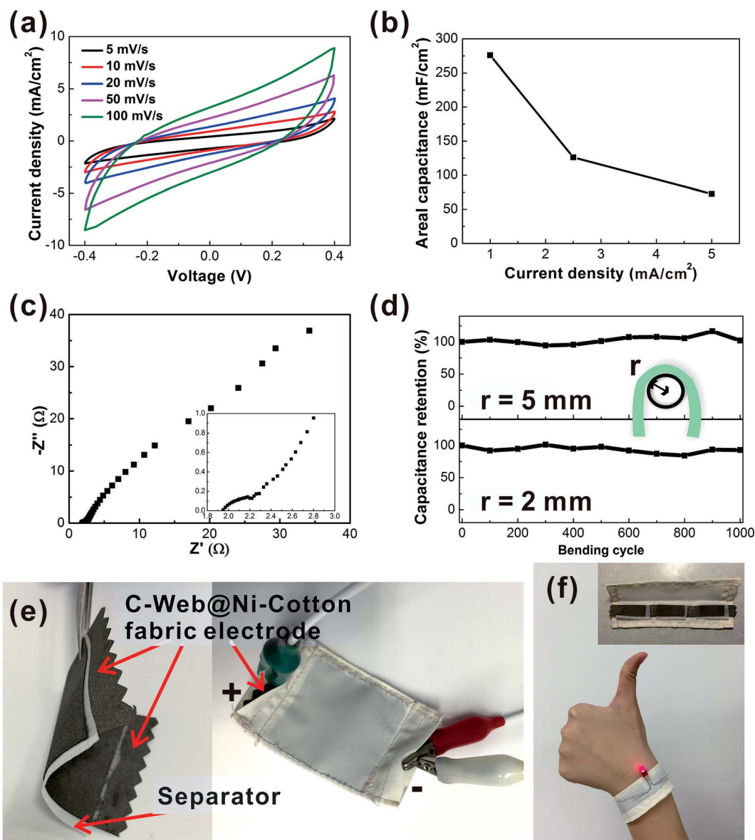
Fig. 4 (a) CV curves of solid-state C-web@Ni-cotton supercapacitor fabric. (b) Summary of the areal capacitance of the supercapacitor fabric at different current densities. (c) Electrochemical impedance spectra (EIS) of the supercapacitor. (d) Capacitance retention of the supercapacitor fabric under different bending radii (scan rate: 50 mV s -1 ). (e) Photographs of a large supercapacitor fabric (active area: 4 cm × 4 cm) enclosed with commercial nonconductive fabrics. (f) Photograph showing that three pieces of supercapacitor fabrics integrated into a wristband can power a LED with 1.6 V turn-on voltage. The inset graph is the structural diagram of the wristband.
