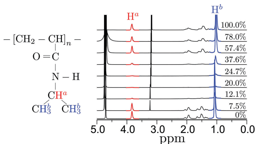
Fig. 5 Left panel shows schematic representation of a monomer of PNIPAm. In NMR experiments we identify the rigidity of H^a and H^b hydrogens as indicated in this schematic. Right panel presents nuclear magnetic resonance (NMR) spectra highlighting H^a and H^b hydrogens as indicated in the left panel. Results are shown for different methanol mole fractions x_m , starting from pure water x_m = 0.0 (or 0%) to pure methanol x_m = 1.0 (or 100%). The signal around 3.75 ppm corresponds to H^a and H^b peak appears around 1.10 ppm. Note that for clear representation of the data, we have aligned the peak positions of H^a . We have used Sigma Aldrich sample of PNIPAm-962.
