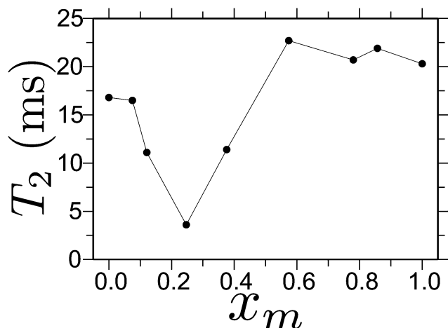
Fig. 6 In-plane relaxation time T_2 of H^+ hydrogen as a function of methanol mole fractions x_m . The data is obtained by integrating the intensity peak around 3.75 ppm in Fig. 5.
