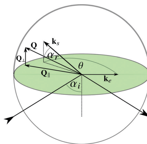
Fig. 1 Scattering geometry of an EWDLS experiment with spherical symmetry.
