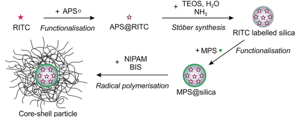
Fig. 12 Schematic illustration of the synthesis of the core–shell particles.
