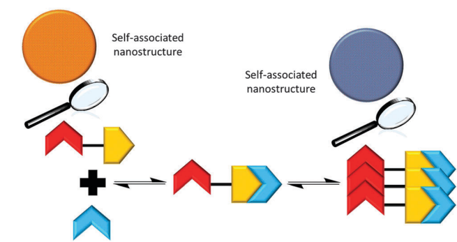
Scheme 3 Summary of the proposed hydrogen bonded complexes formed from solutions of 1 and solutions of 1 and 2 in \text{DMSO} , based on the NMR evidence presented herein.
