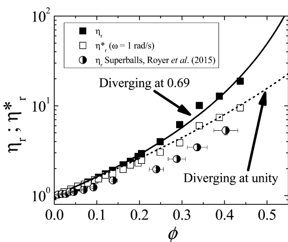
Fig. 9 Low shear steady (closed) and complex (open) viscosity as a function of the volume fraction of cubic particles. The solid and dotted lines are fits to the steady shear viscosity and complex viscosity, respectively, using a modified Eilers equation with an adjustable power law exponent. The half-filled circles mark the low shear viscosity under steady shear for suspension of superballs as measured by Royer et al. 45
